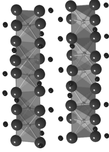
Gibbsite
