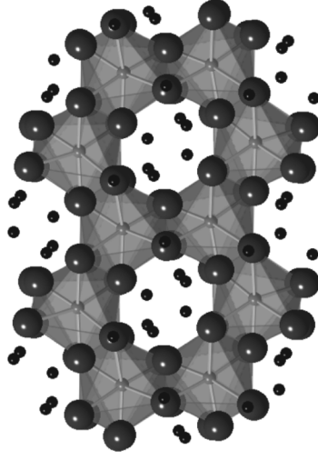
Diocahedral
