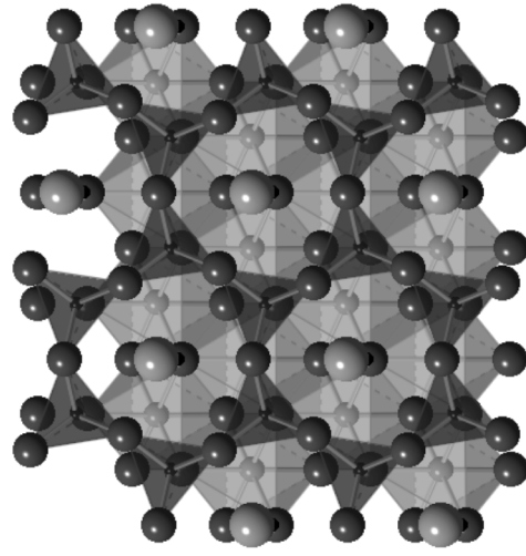
Trioctahedral
