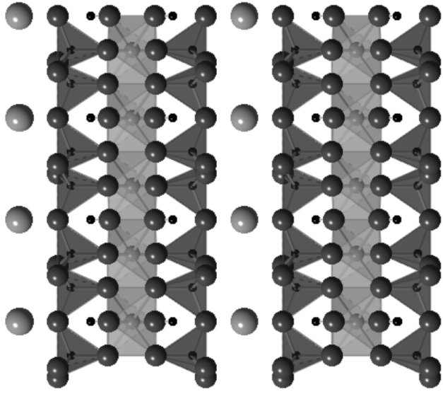
Phlogopite
