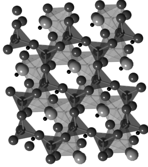
Diocahedral
