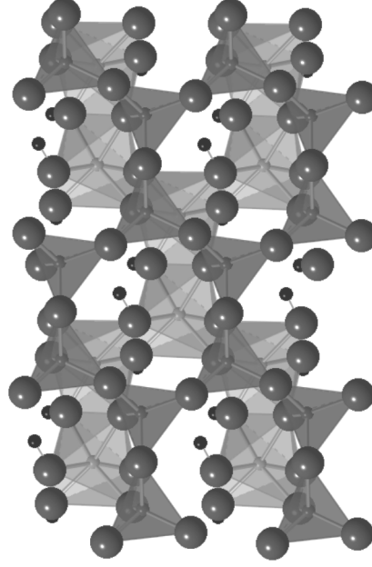
Dioctahedral
