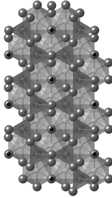
Trioctahedral
