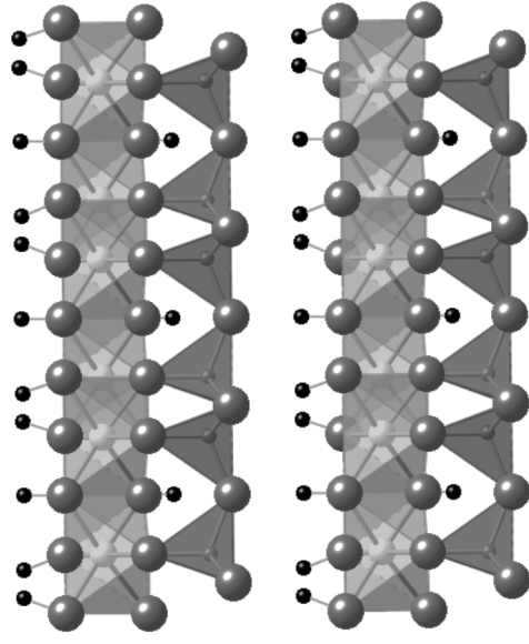
Lizardite (Serpentine Group)
